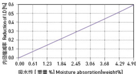
Graph HPP13-9: Effect of moisture absorption on HPP13 bearings
