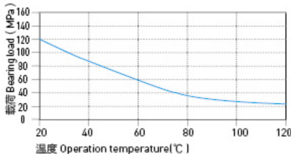
Graph HPP13-3: Load-Temperature diagrams
