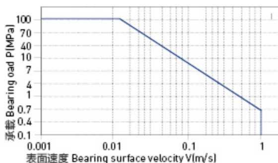
Graph HPP13-1: Permissible PV value for HPP13
