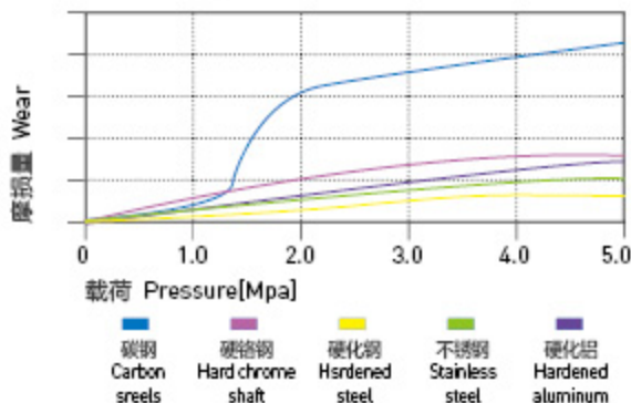
图表 HPP13-8: 旋转磨损随轴材料与压力变化关系 v=0.2\text{m/s} Graph HPP13-8: The bearing wear & pressure under rotating with different shaft materials, v=0.2\text{m/s}
