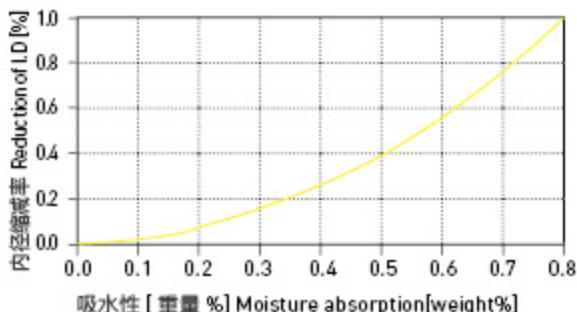
图表 HPP7-9: 吸水性的影响 Graph HPP7-9: Effect of moisture absorption on HPP7 bearings
