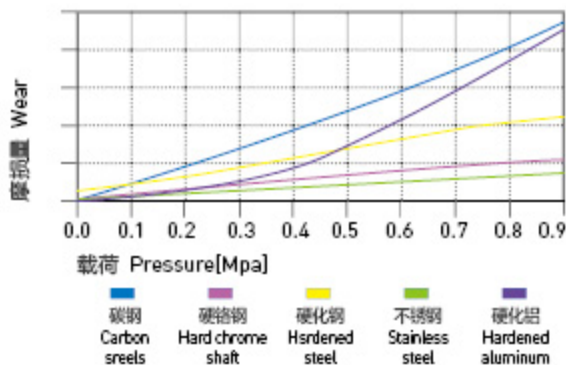
图表 HPP7-8: 旋转磨损随轴材料与压力变化关系 v=0.2\text{m/s} Graph HPP7-8: The bearing wear & pressure under rotating with different shaft materials, v=0.2\text{m/s}
