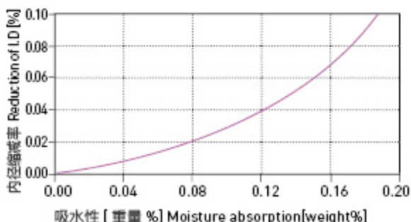
图表 HPP24-9: 吸水性的影响 Graph HPP24-9: Effect of moisture absorption on HPP24 bearings
