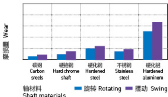
图表 HPP24-8: 旋转磨损随轴材料与压力变化关系 v=0.2m/s Graph HPP24-8: The bearing wear & pressure under rotating with different shaft materials, v=0.2m/s
