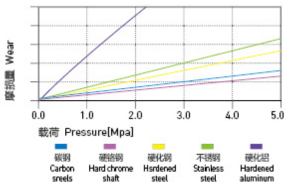
图表 HPP24-8: 旋转磨损随轴材料与压力变化关系 v=0.2m/s Graph HPP24-8: The bearing wear & pressure under rotating with different shaft materials, v=0.2m/s
